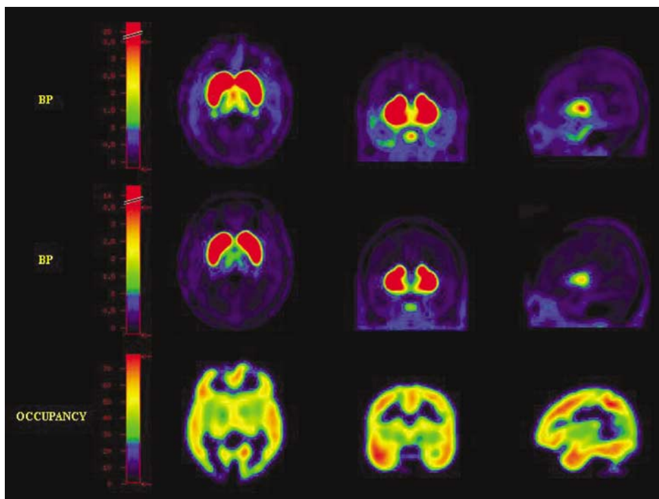
Figure 3 Parametric mean BP images in normal volunteers ( n = 7 , top row) and in clozapine-treated patients ( n = 15 , middle row). The bottom row illustrates the D_2/D_3 receptor occupancy in each single voxel in the patient group, clearly demonstrating the significantly higher binding in cortical regions compared to the striatum.
