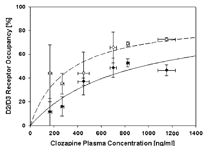
Figure 1 Relationship between clozapine plasma levels (x-axis) and dopamine D_2/D_3 receptor occupancy in the putamen (y-axis, filled circles, solid line) and in the inferior temporal cortex (open circles, dashed line) in 15 patients with schizophrenia and schizoaffective disorder receiving therapeutic doses of clozapine. For illustrative purposes, plasma concentrations were averaged stepwise (0–199, 200–399, 400–599 ng/ml, etc) and, together with their corresponding occupancy values, presented as means \pm SEM. However, statistical values presented in the text are based on individual values.
